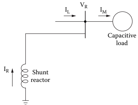
Figure 3.10 Shunt-reactor-compensated load. (From [1]. Used with permission.)
