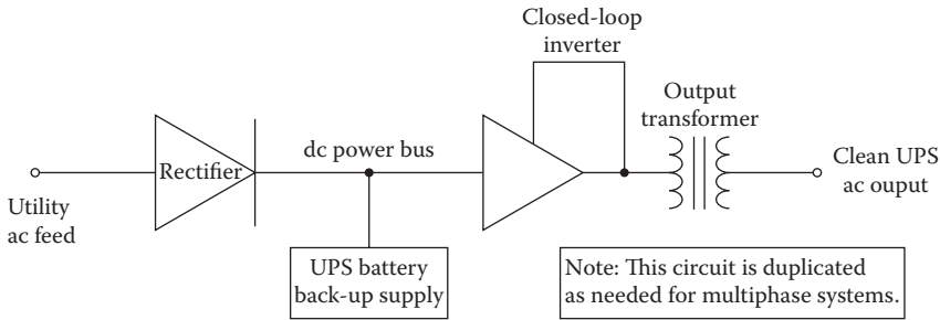
Figure 13.5 Block diagram of an uninterruptible power system using ac rectification to float the battery supply. A closed-loop inverter draws on this supply and delivers clean ac power to the protected load.
