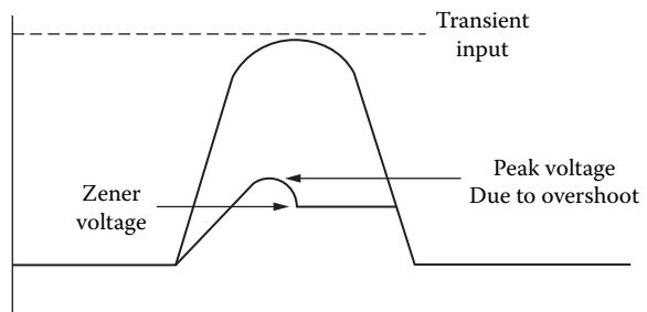
Figure 15.13 Transient clamp overshoot resulting from inductive effects of the wiring system. (Courtesy of Motorola.)
