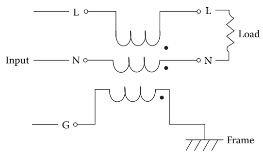
Figure 15.1 Balun common-mode filter. (After [1].)
