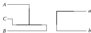
Figure 4.23 The T-connection for a three-phase to two-phase transformation. (From [7]. Used with permission.)
