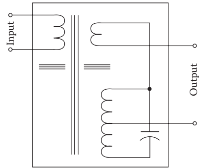
Figure 14.1 Basic design of a ferroresonant transformer. (After [1].)
