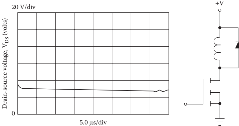
Figure 6.8 Drain-source transient with a clamping diode across the inductive load. (Courtesy of Motorola.)
