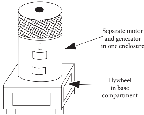
Figure 12.5 Vertical m-g set with an enclosed flywheel. (After [1].)
