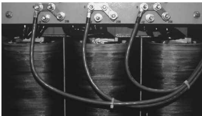
Figure 4.24 A medium-power, three-phase transformer.
